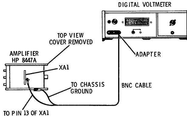
Figure 5-1. Power Supply Voltage Adjustment Test Setup
